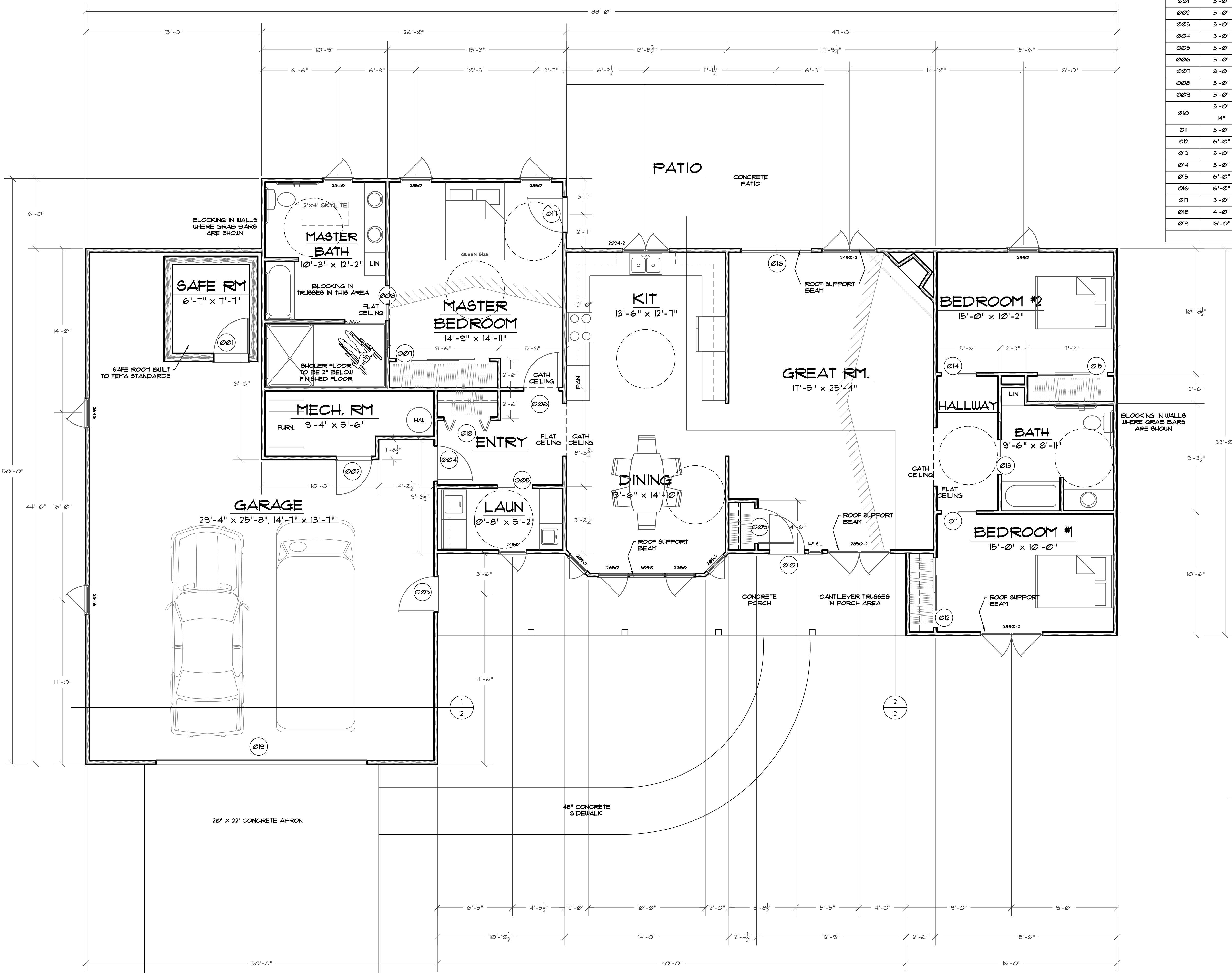
FLOOR PLAN 2078 SQ.FT. FINISHED AREA
